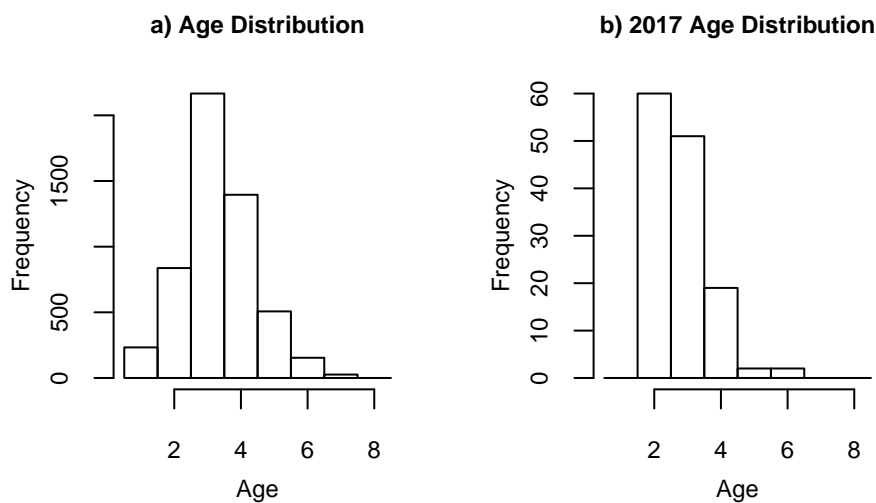
Figure 10. Age-distribution of the spawning population of Arctic grayling in Red Rock Creek for a) all years of data (1994–2017, with missing years), and b) 2017.
