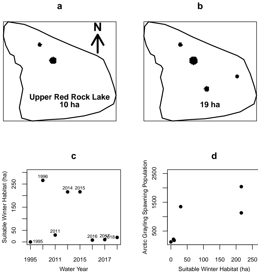
Figure 11. a) Extent of minimum area of suitable Arctic grayling winter habitat in Upper Red Rock Lake, 2017, b) 2018, c) annual estimate of minimum area of suitable habitat for water years 1995–2018, and d) grayling spawning population as a function of minimum area of suitable winter habitat for years when both were estimated.
