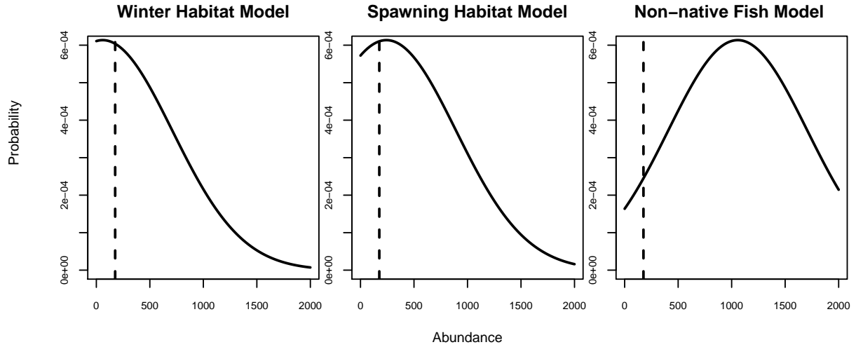
Figure 8. Normal probability density plots for Winter Habitat , Spawning Habitat , and Non-native Fish models with \mu = 60, 243, and 1057, respectively. Standard deviation for all plots = 650. Vertical dashed lines show the observed grayling spawning population, \hat{N} = 176, in 2017.
