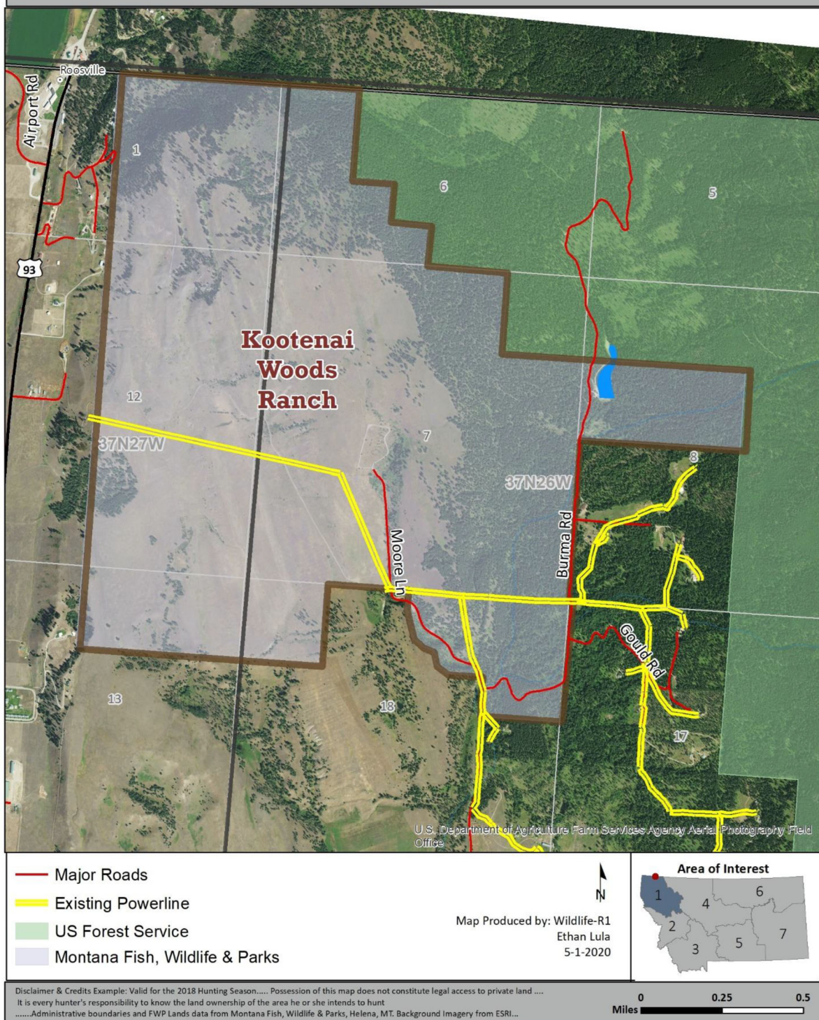
Figure 1. Existing Powerlines on WRWMA
